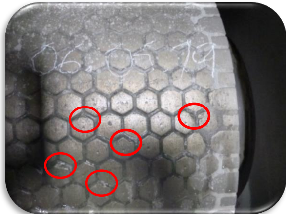
Such damages due to the passage of foreign metal do not require maintenance as the cracks do not propagate due to multi-metal composite.
